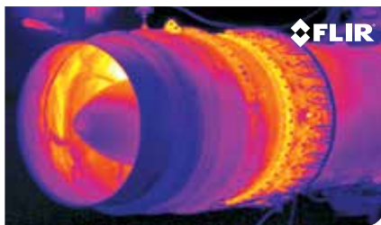
Jet engine
